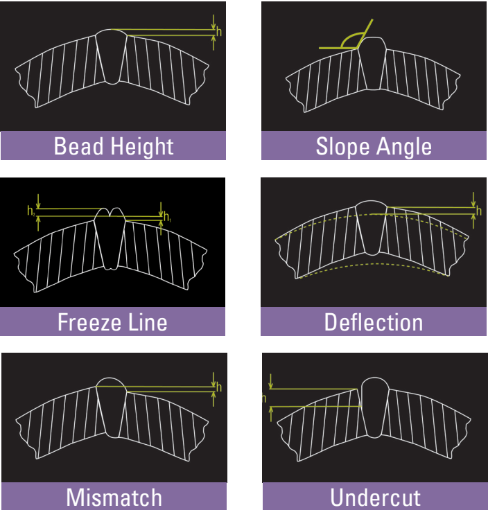
Weld Defects
