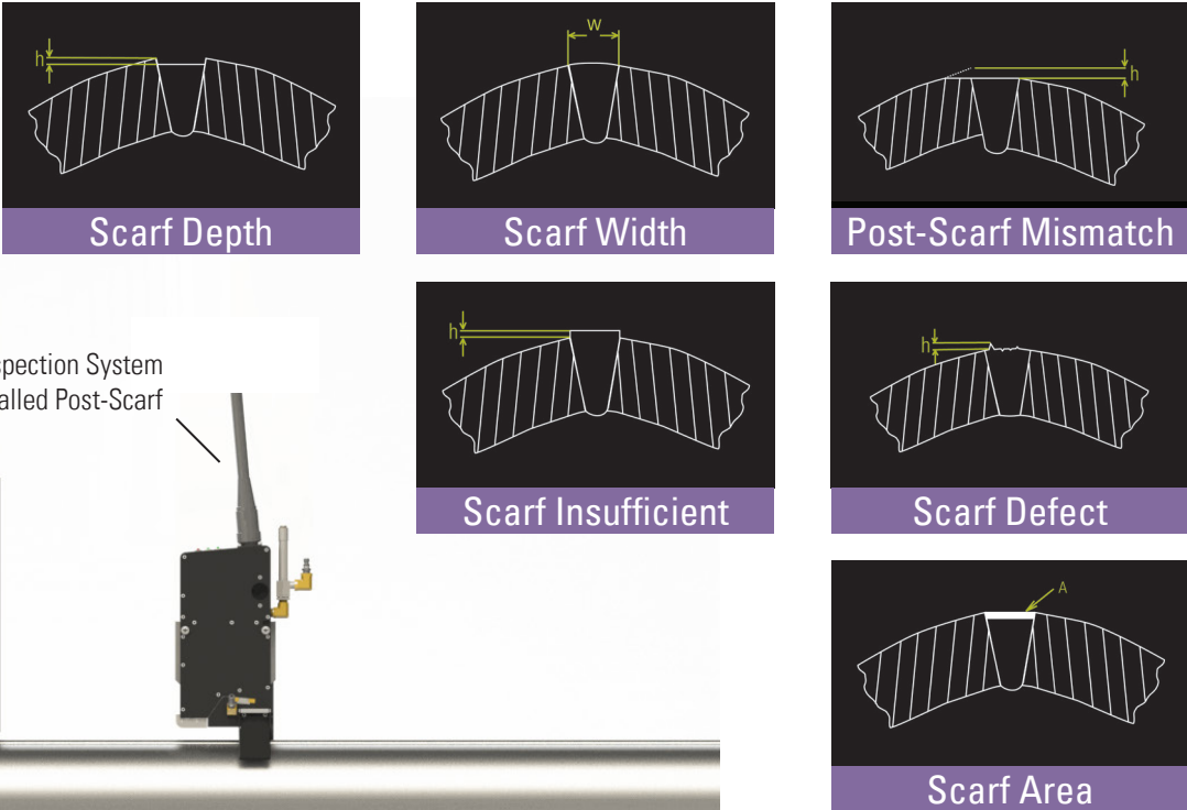
Scarf Defects
